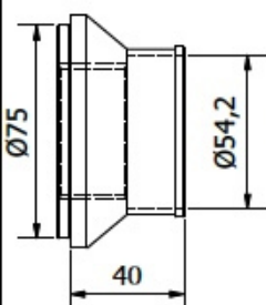
Ø54,2 PIPE BRAZING CONNECTION Ø70,2 PIPE BRAZING CONNECTION
