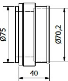
Ø54,2 PIPE BRAZING CONNECTION Ø70,2 PIPE BRAZING CONNECTION
