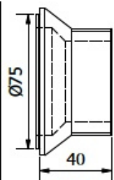
MALE OUTSIDE THREAD ISO7-R 2"
